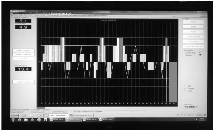
Figure VII: Cross Direction Web Profile
