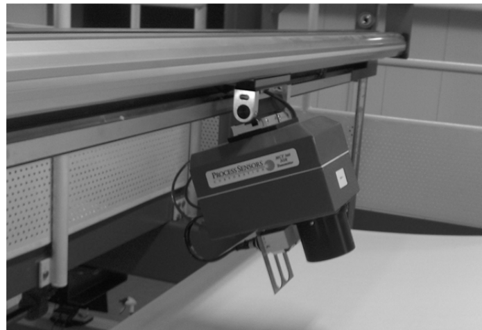
Figure VI: NIR Moisture Transmitter On Paper Web
