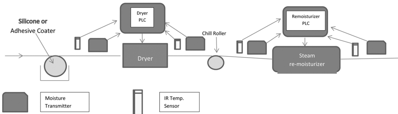
Figure XI: Flow Chart Re-Moisturizer
