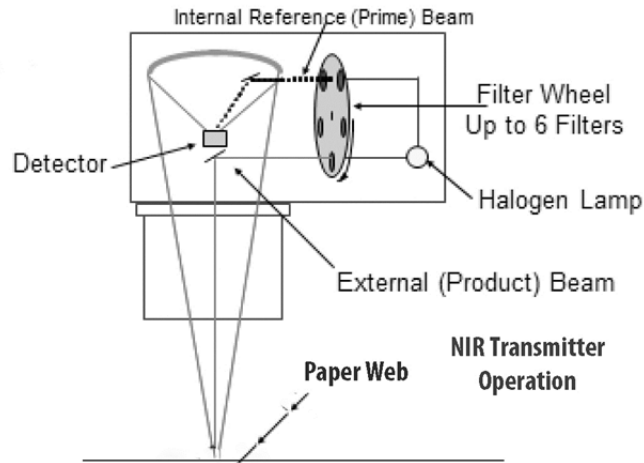
Figure V: Workings of an NIR Transmitter
