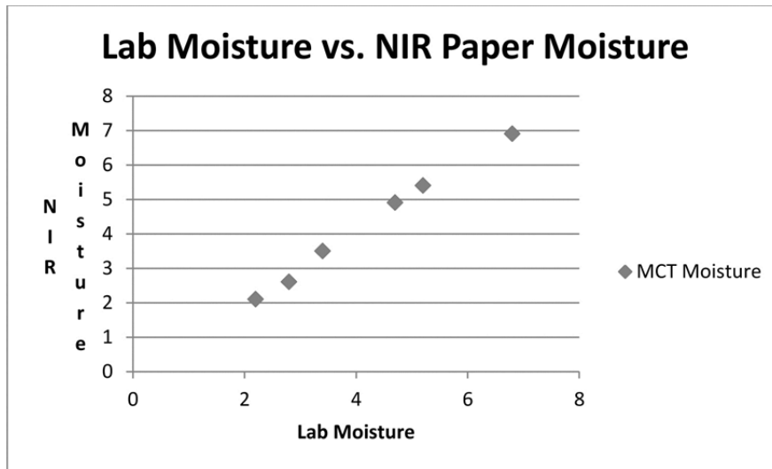
Figure X: Paper Moisture Measurement Comparison
