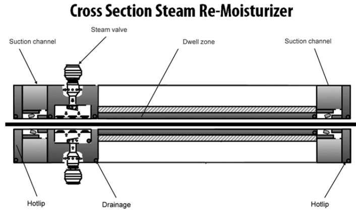
Figure II: Cross Direction Steam Re-Moisturizer
