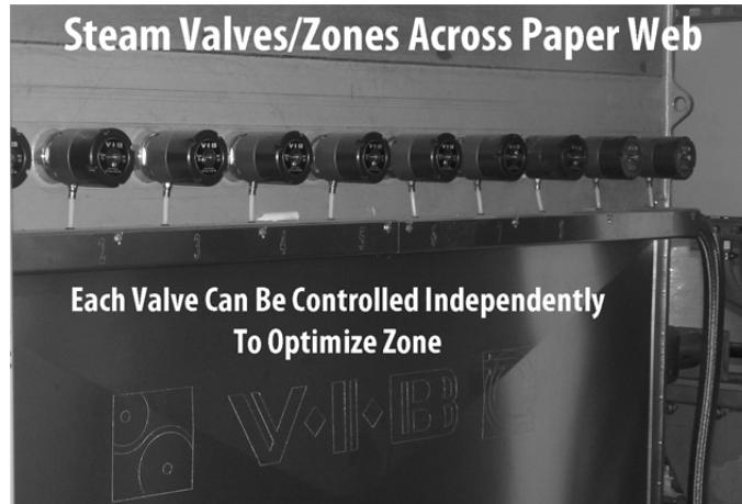
Figure IV: Steam Valves and Zones in Re-Moisturizer
